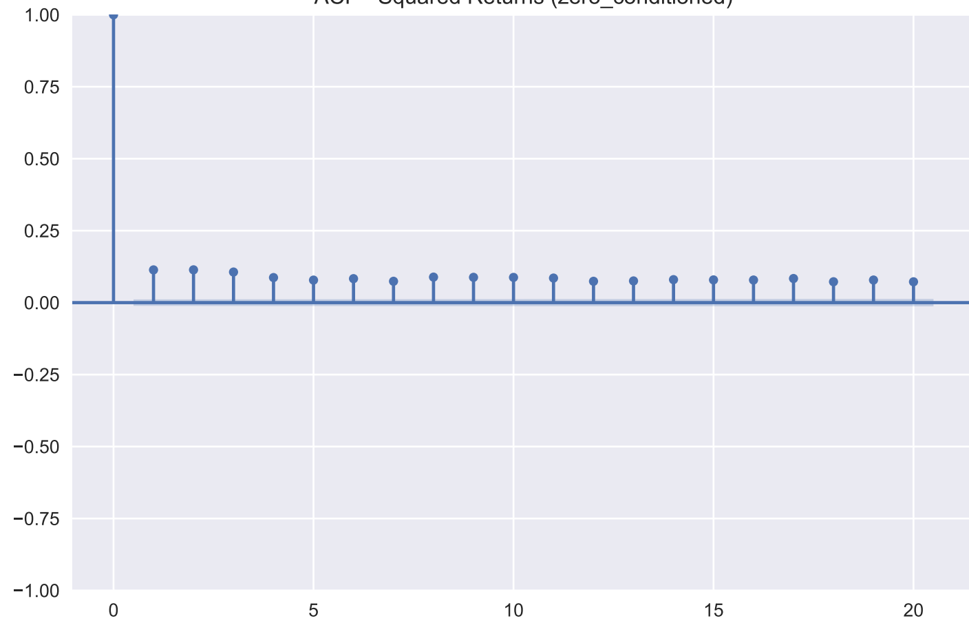
ACF - Squared Returns (zero_conditioned)
