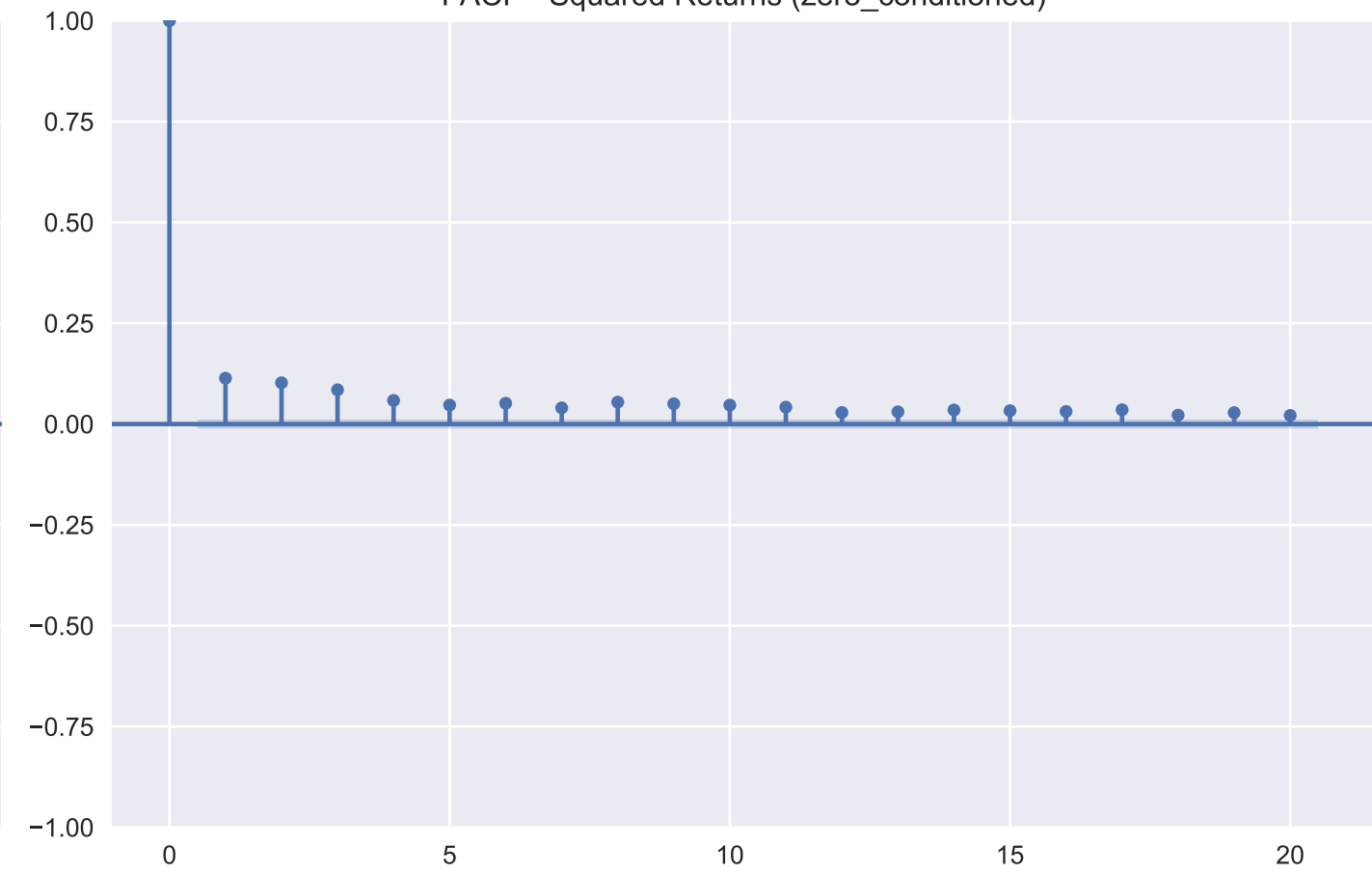
PACF - Squared Returns (zero_conditioned)
